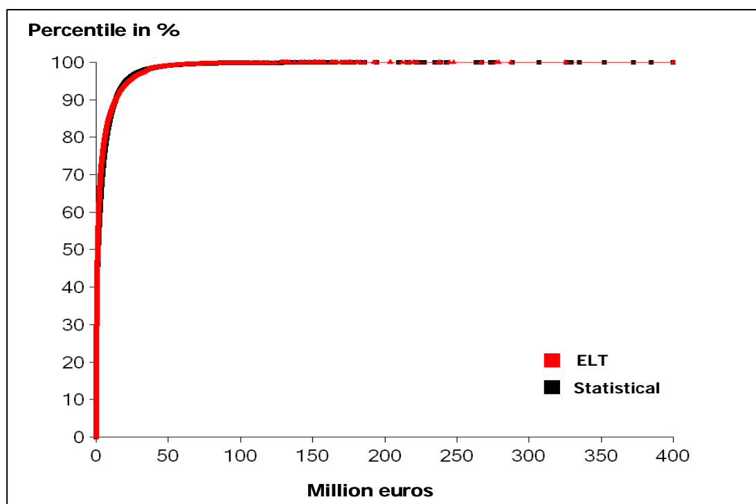
Figure 5a: Annual storm loss distribution according to the mathematical statistical model (black) vs. modelling based on natural-risk models (red)
