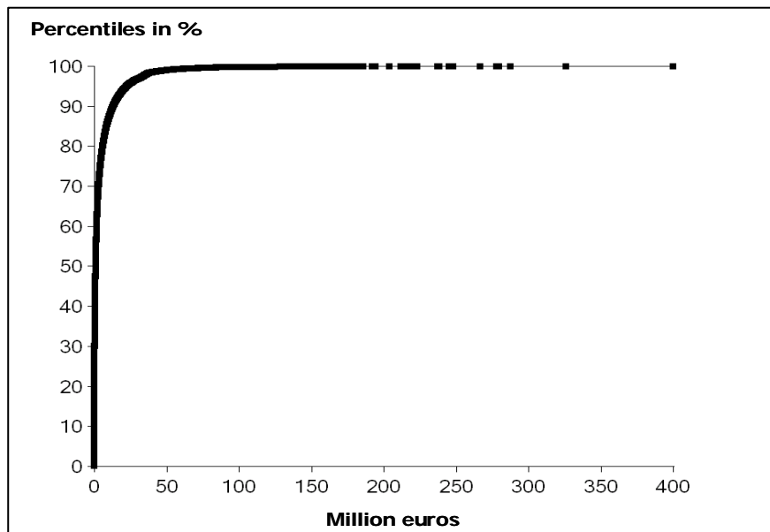
Figure 3a: Annual storm loss distribution
