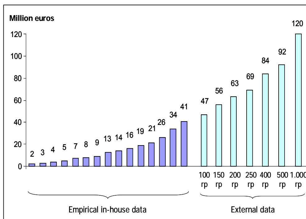
Figure 4a: Empirical in-house data for annual storm claims and external data for long return periods (rp)
