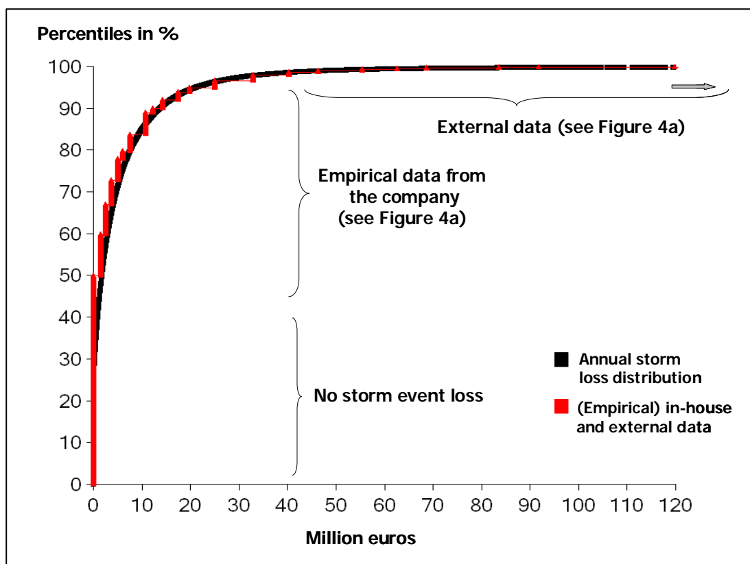
Figure 4b: Annual storm loss distribution vs. empirical distribution (in-house and external data from Figure 4a)
