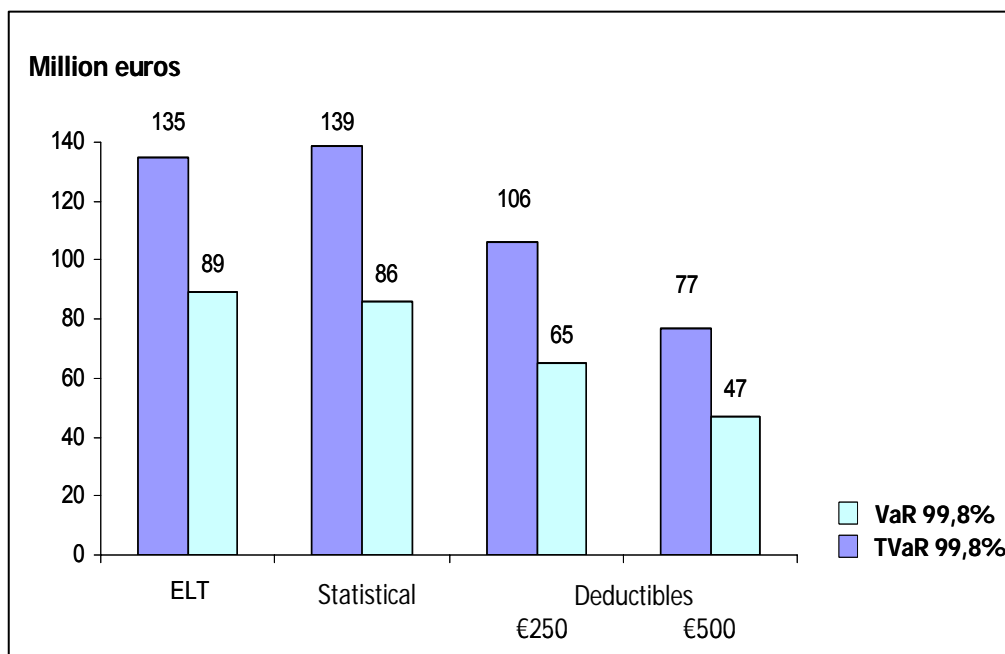
Figure 6: Value-at-risk and Tail-value-at-risk at a confidence level of 99.8% for annual storm loss
